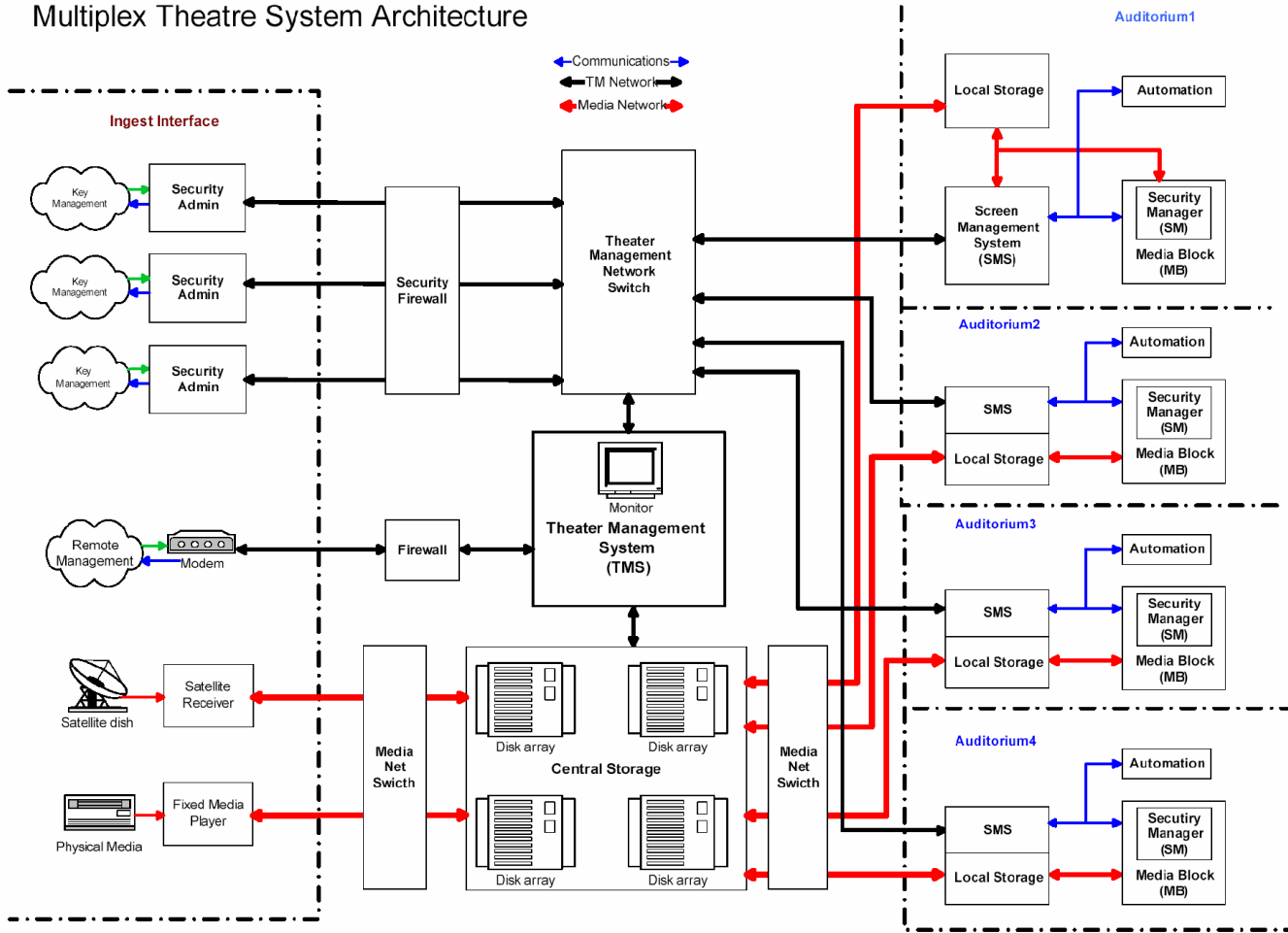
Figure 13: Multiplex Theater System Architecture
