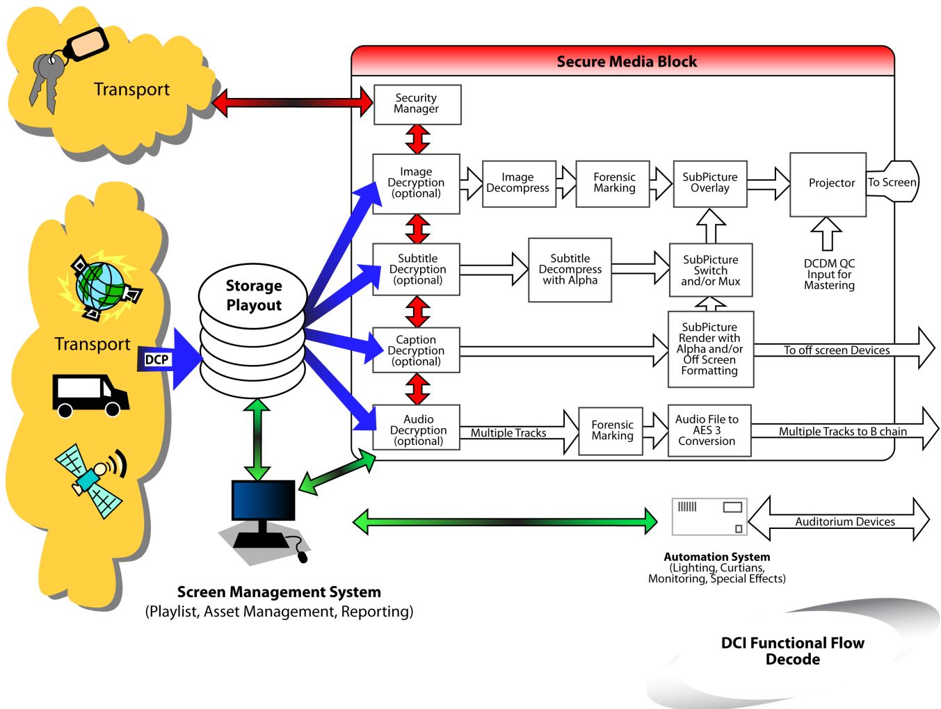
Figure 2: System Overview Functional Decode Flow
