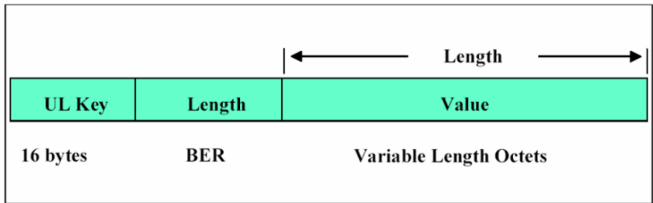
Figure 9: Example of KLV Coding
